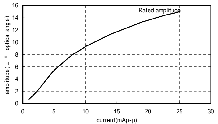
Characteristics of Current-amplitude (Outside / DC driving)
