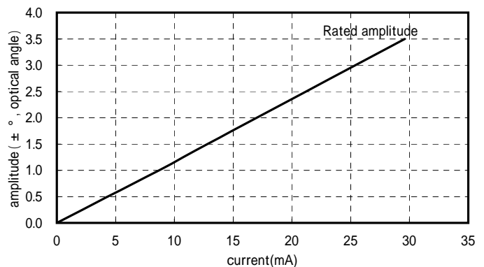
Characteristics of Current-amplitude (Outside / DC driving)
