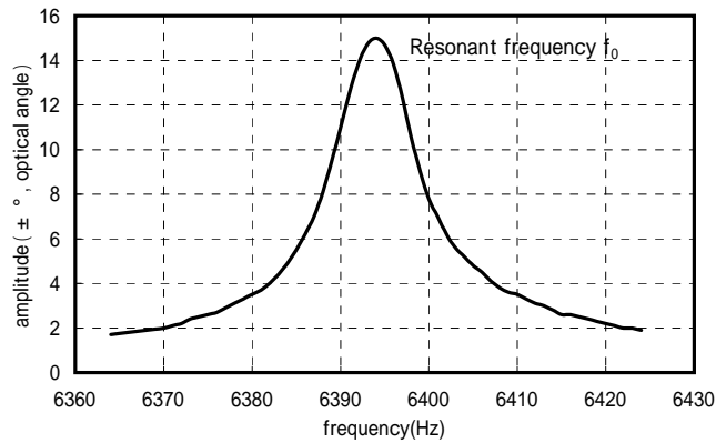
Characteristics of frequency-amplitude (Inside / Sine wave driving)
